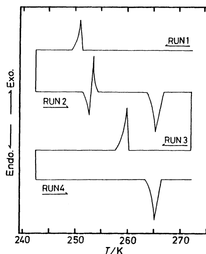
Fig. 1. DTA curves of RbNO 2 showing the stable-stable and metastable-stable transitions.
